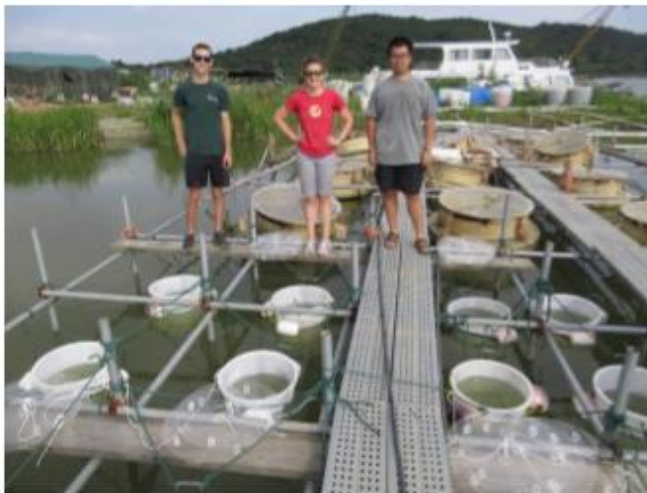
Experimental mesocosms on the shoreline of Lake Taihu, used to examine nutrient-cyanobacterial bloom potentials. Shown are PhD Graduate Students (from left to right), Bryce Van Dam (PhD in Marine Science, UNC-CH, May 2018), Alexandria Hounshell (PhD in Marine Science UNC-CH, expected in May, 2019) and Kaijun Lu (PhD in Marine Science, Univ. of Texas, expected May, 2019).
