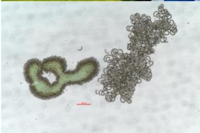
Photomicrograph of dominant cyanobacterial bloom genera found on Lake Taihu, China. On the left is a colony of the non N_2 fixer Microcystis and on the right is a colony of the N_2 fixer Dolichospermum (formerly Anabaena ). Photographed by P.I. Hans Paerl during a July 2018 bloom
